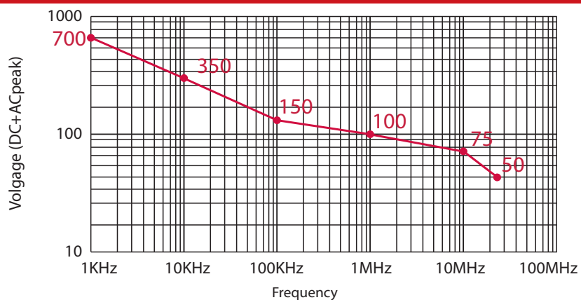
Derating Curve
