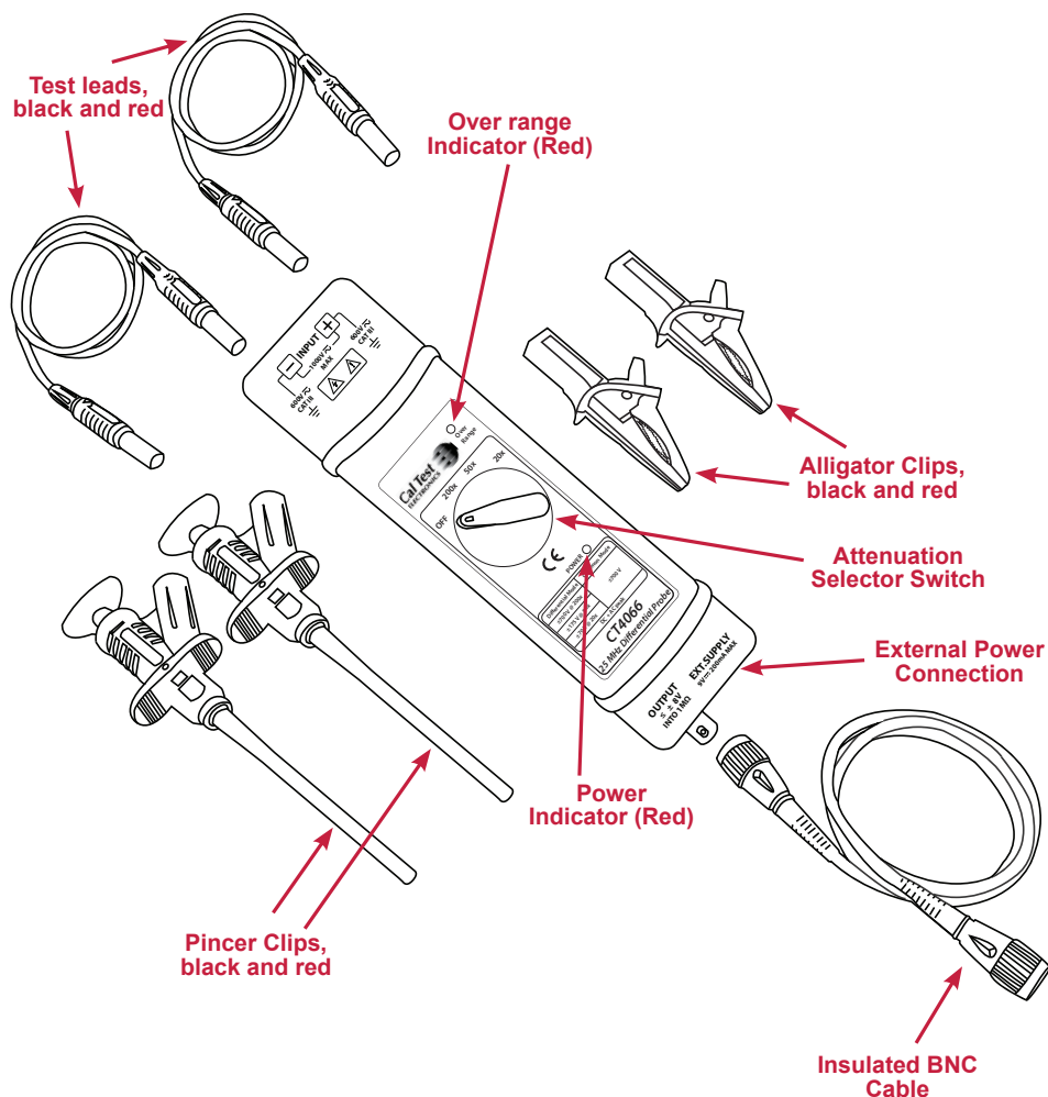
Figure 1 CT4066: Front Panel Features
