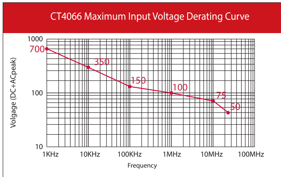
Figure 2 CT4066: Derating Curve
