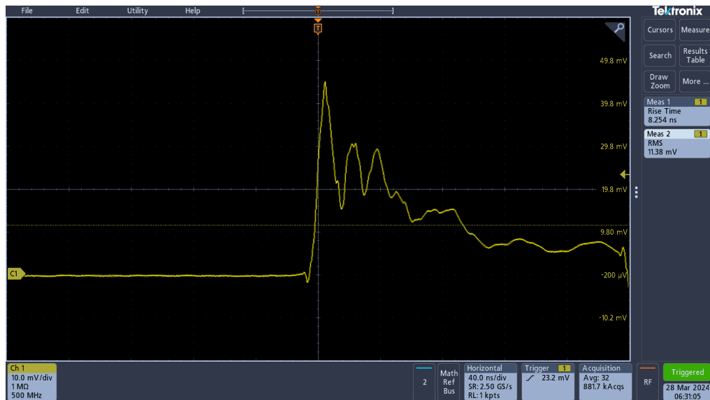
Figure 4 Rise Time
