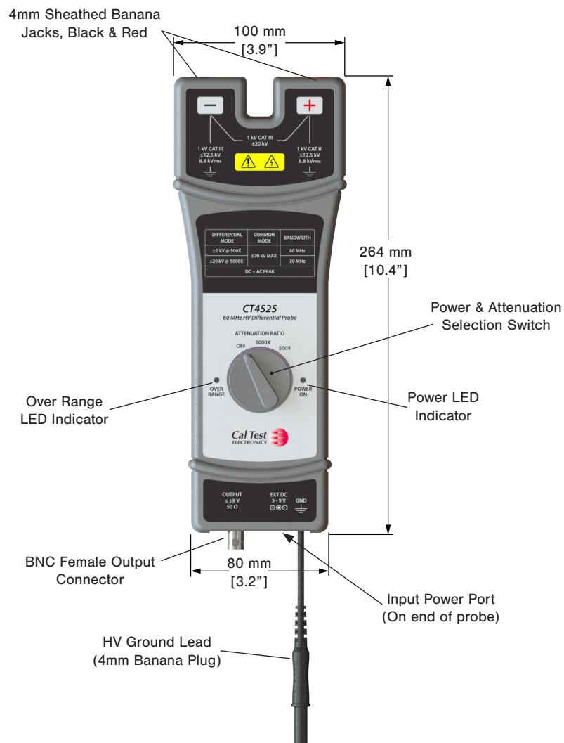
Figure 1 Probe Details
