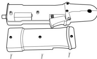
Figure 5: Installation de la pile
