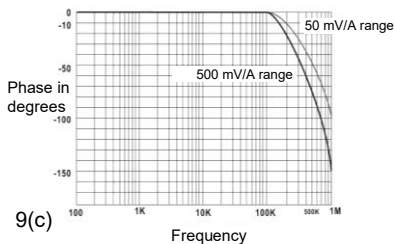
Figure 9(a - d): Phase versus Frequency @ 1 A peak, typical
