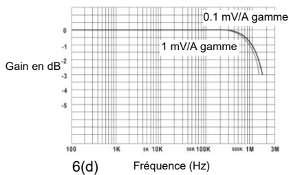
Figure 6(a – d): Courbe Gain/Fréquence @ 1 A crete, typique
