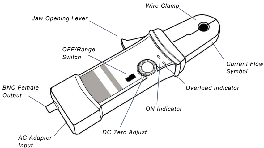
Figure 1: Controls and indicators on current probe
