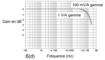
Figure 6(a – d): Courbe Gain/Fréquence @ 1 A crete, typique
