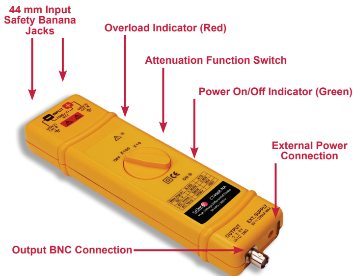
Figure 1 Front Panel Features
