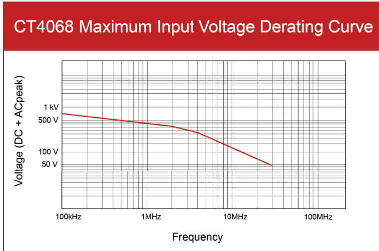
Figure 1 CT4068-NA Derating Curve
